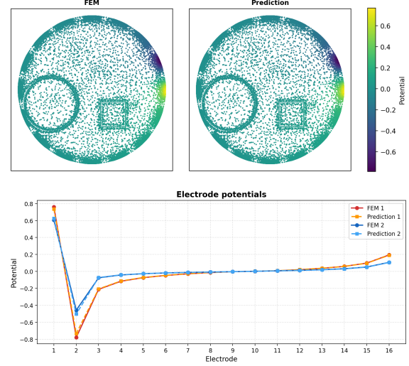
Fig. 1: Comparison of electrical potentials obtained from FEM simulations and from the surrogate model. The upper panel shows the electrical potential distributions on the cylindrical volume mesh for a single conductivity distribution, the lower panel shows the corresponding electrode potentials for two different conductivity distributions. The respective conductivity distributions were not part of the training set. The cylindrical domain has dimensions R = 0.14 m and h = 0.07 m. The background conductivity is set to 1 \text{ S m}^{-1} and the objects have conductivities \gamma_{\text{cylinder}} = 100 \text{ S m}^{-1} and \gamma_{\text{cuboid}} = 63 \text{ S m}^{-1} .
