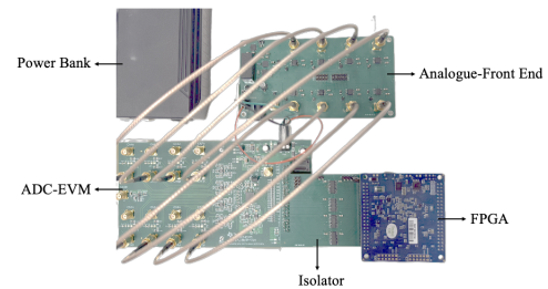
Fig. 1: FPGA-based high-speed fnEIT system hardware.
